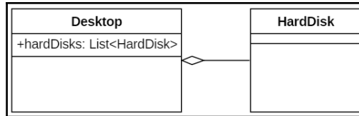
Aggregation example
