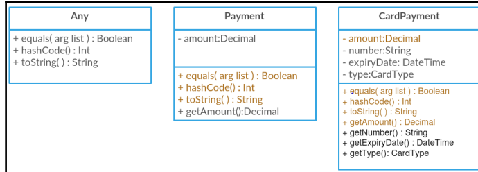
Simple inheritance
