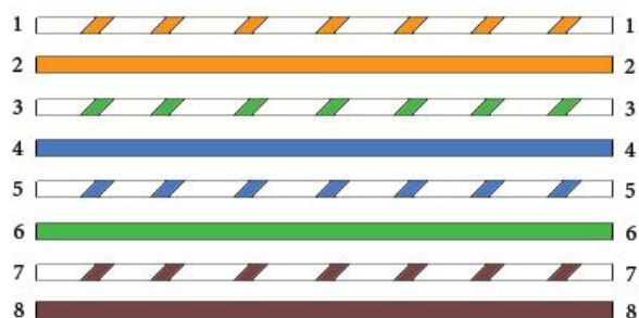
Straight Through Wiring Guide 568-B
